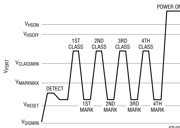
Figure 5. Type 3 or Type 4 PSE, 4-Event Class Sequence
