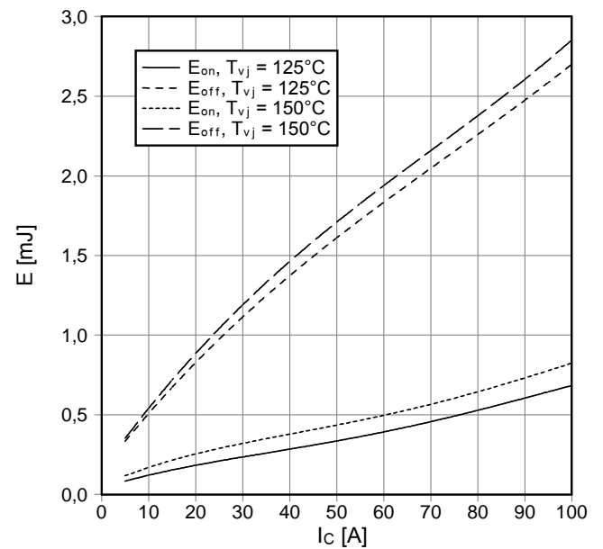
Schaltverluste IGBT-Wechselr. (typisch) switching losses IGBT-inverter (typical) E_{on} = f(I_C) , E_{off} = f(I_C) V_{GE} = \pm 15\text{ V} , R_{Gon} = 8,2\ \Omega , R_{Goff} = 8,2\ \Omega , V_{CE} = 300\text{ V}
