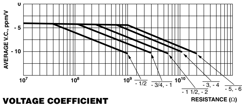
VOLTAGE COEFFICIENT
