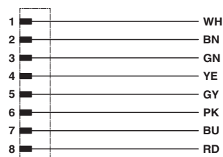
Contact assignment of the M8 plug
