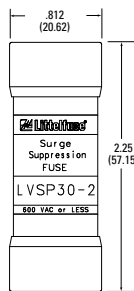
Figure 2: Cartridge 30-80 A
