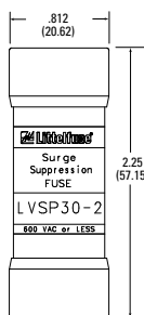
Figure 2: Cartridge 30-80 A
