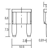
Low Profile MINI dimensions in mm (inches)
