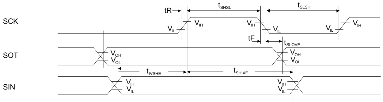
Slave mode
