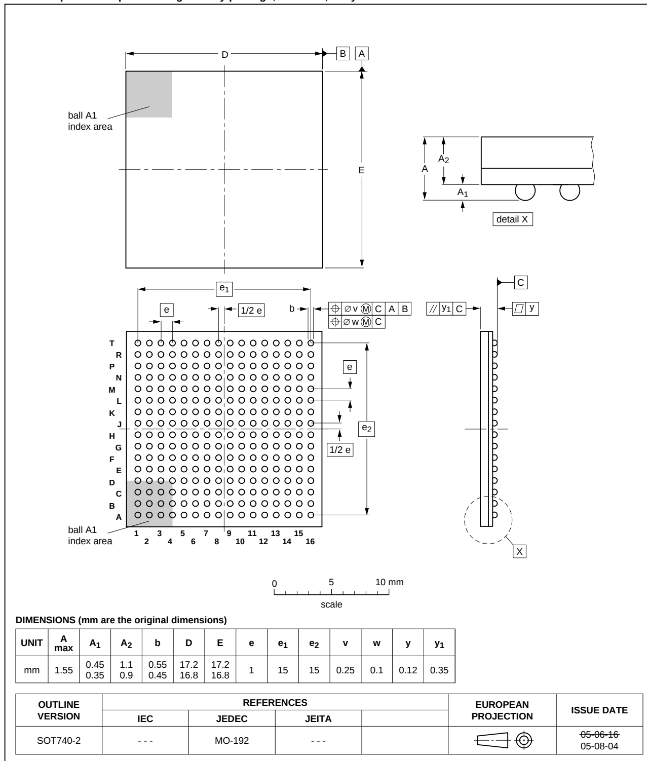
Fig 45. Package outline of the LBG A256 package
