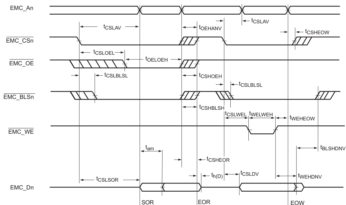
Fig 32. External static memory read/write access (PB = 1)
