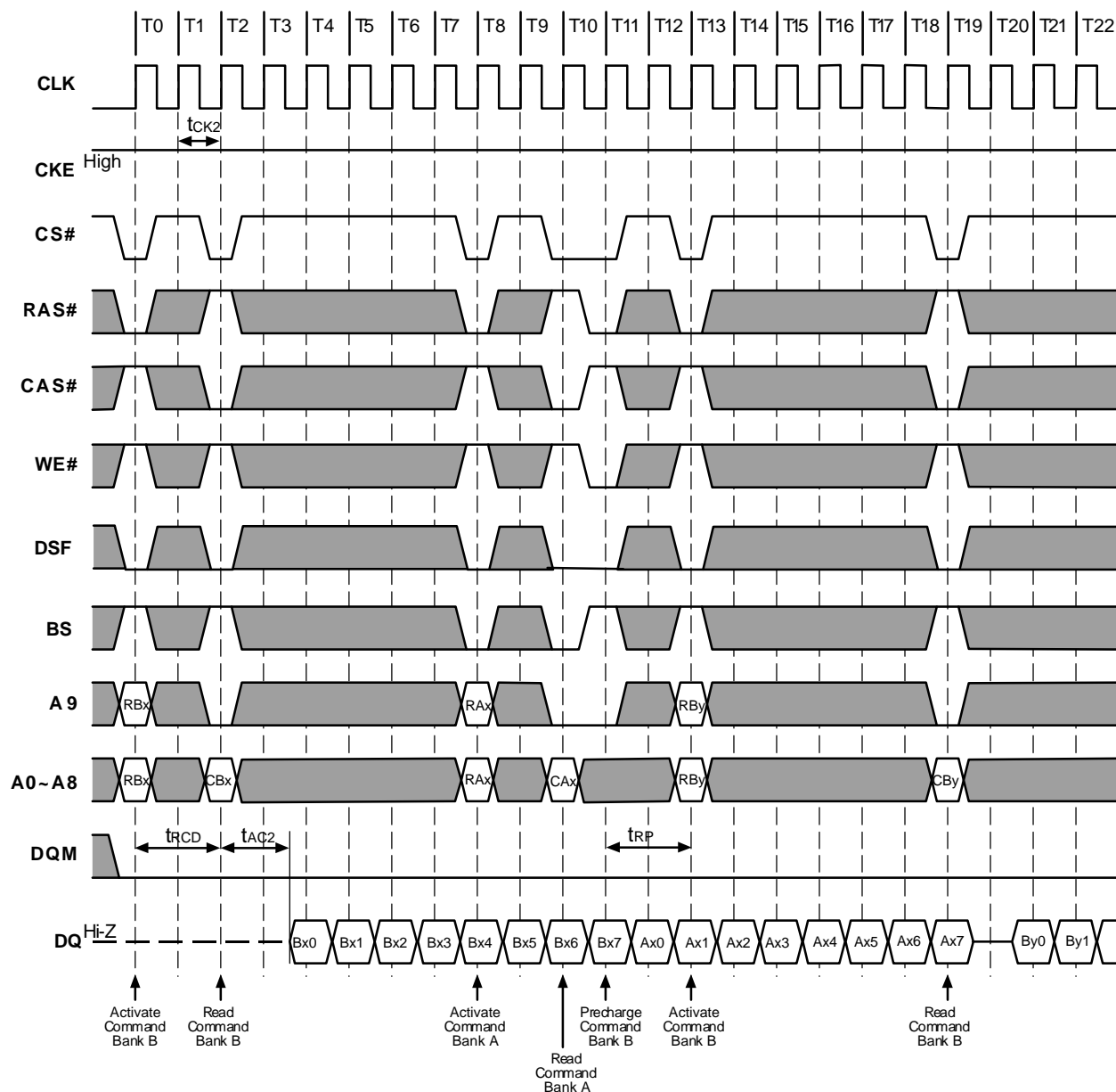
Figure 11.2. Random Row Read (Interleaving Banks) (Burst Length=8, CAS# Latency=2)
