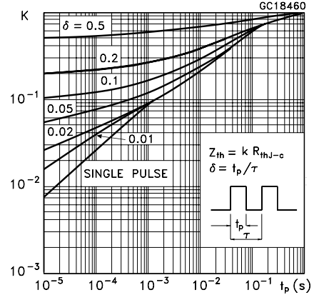
Figure 3: Thermal impedance
