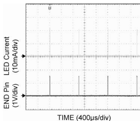
Figure 6. PWM Signal at 1% Duty Cycle ( I_{avg} = 0.2\text{mA} )
