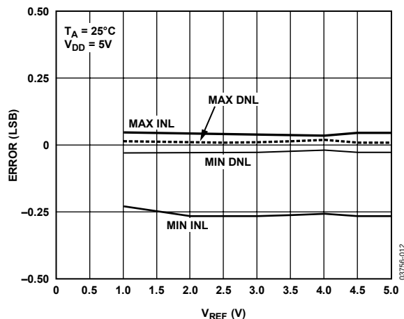
Figure 10. AD5337 INL and DNL Error vs. V_{REF}
