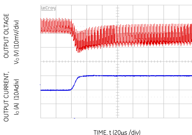
Figure 4. Transient Response to Dynamic Load Change from 50% to 100% at 12Vin, C_{out} = 1 \times 47 \mu\text{F} + 11 \times 330 \mu\text{F} CTune=47nF, RTune=178 ohms
