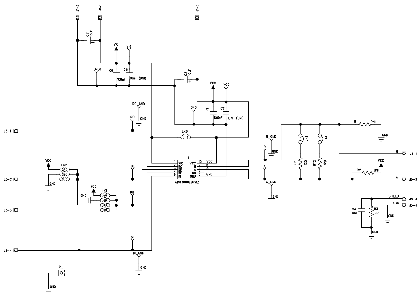
Figure 5. EVAL-ADM3066EBZ Schematic
