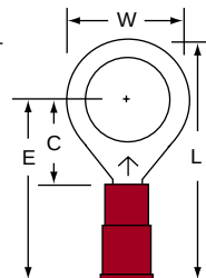
MNG18-38R Stud Size 3/8 Wire Range 22-18
