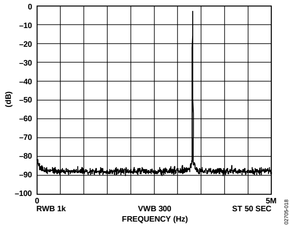
Figure 20. f_{MCLK} = 10 \text{ MHz} ; f_{OUT} = 3.33 \text{ MHz} = f_{MCLK}/3 , Frequency Word = 555555
