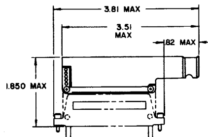
2 INCH PLUG ASSY INSTALLATION DATA REF
