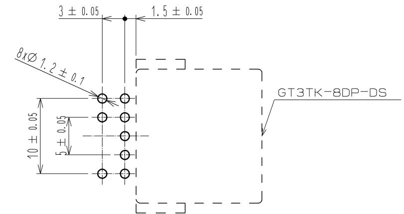
RECOMMENDED PCB BOARD LAYOUT
