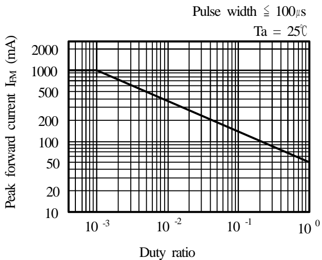
(Fig.7) Forward current vs. duty ratio
