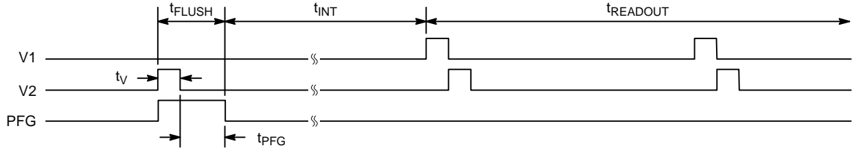
Figure 21. Pulse Flush Gate Timing
