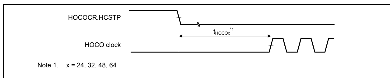
Figure 2.27 HOCO clock oscillation start timing (started by setting the HOCOxR.HCSTP bit)
