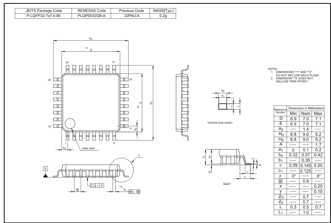
Figure 1.3 LQFP 32-pin
