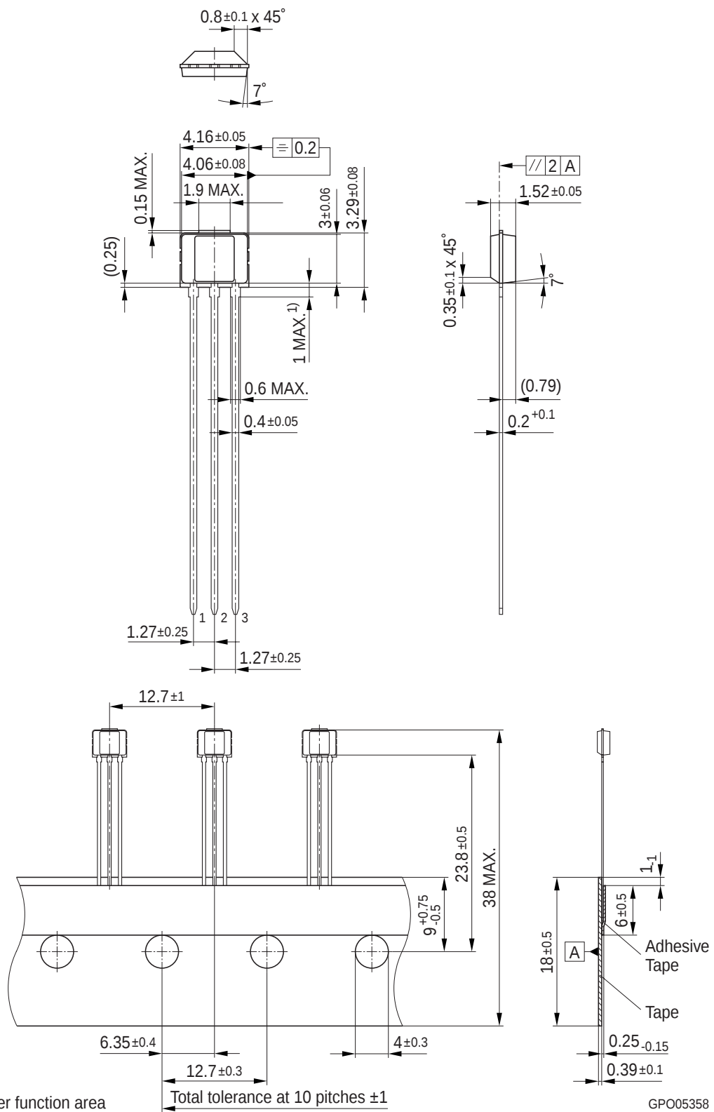
Figure 8 PG-SSO-3-2 Package Outline
