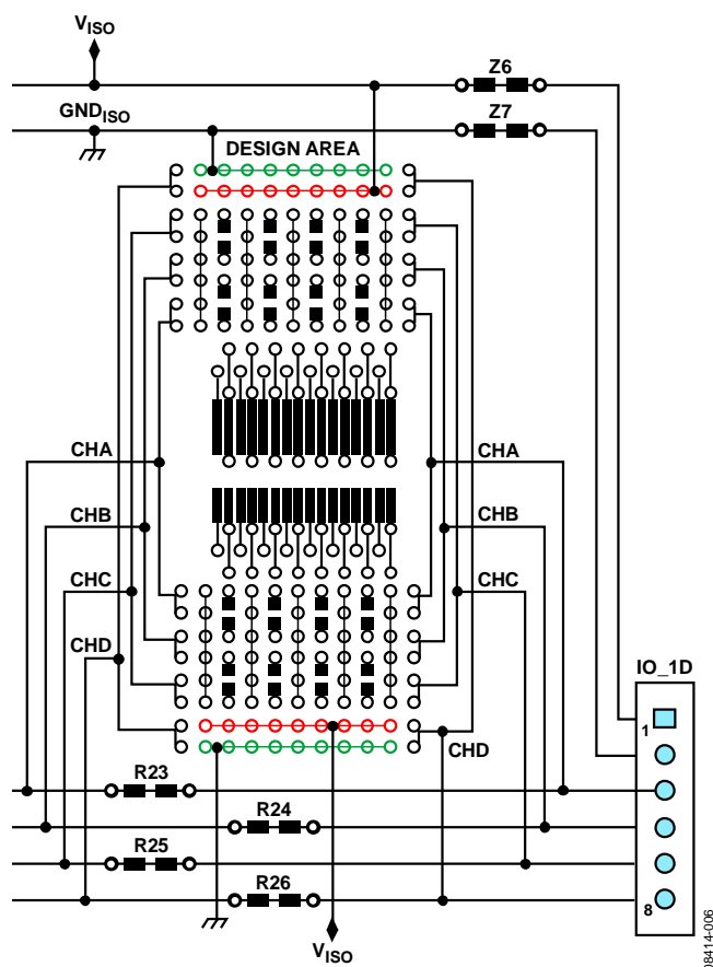
Figure 6. Design Area
