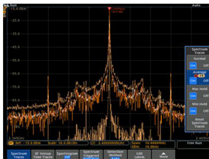
Normal, Average, Max Hold, and Min Hold spectrum traces
