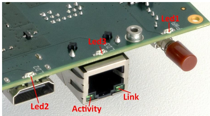
Figure 45: Carrier LEDs
