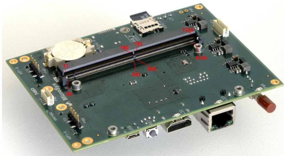
Figure 27: MXM-Connector
