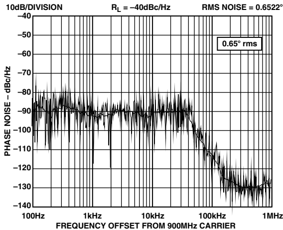
TPC 3. ADF4213 Integrated Phase Noise (900 MHz, 200 kHz, 35 kHz, Typical Lock Time: 200 \mu s )
