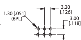
P.C. MOUNTING
