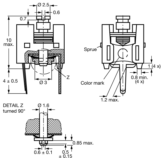
Trimmers BFC2 809 090.. series, with one rotor contact
