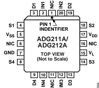
Figure 4. PLCC Pin Configuration
