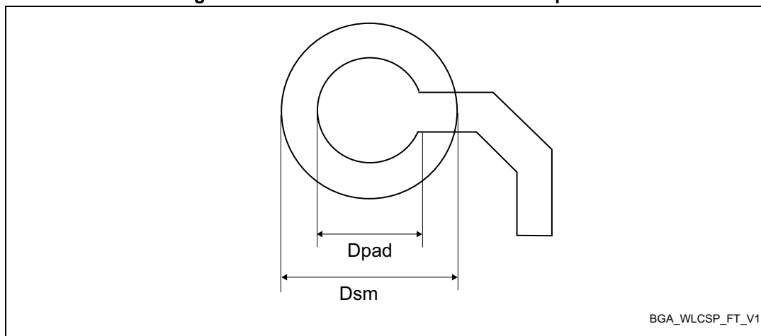
Figure 69. TFBGA100 - recommended footprint
