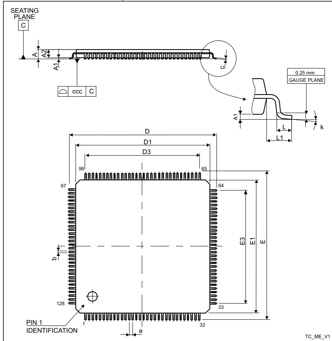
Figure 74. LQFP128 - outline
