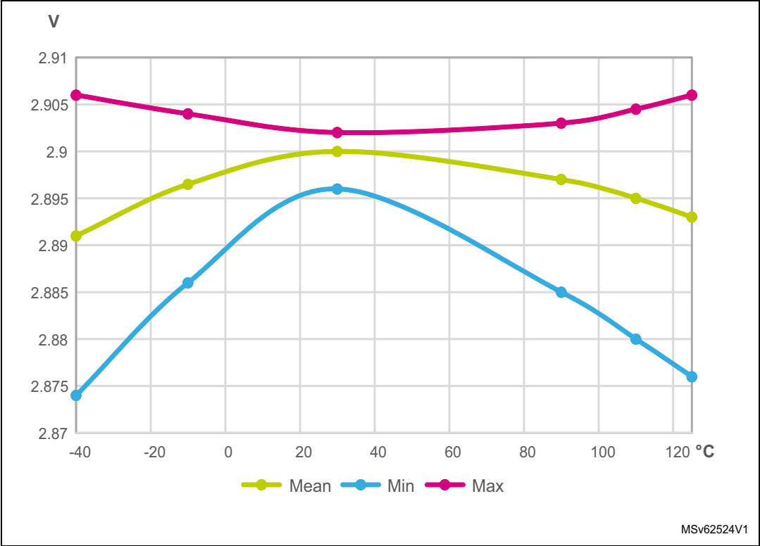
Figure 33. V_{\text{REFOUT}} TEMP in case VRS = 10
