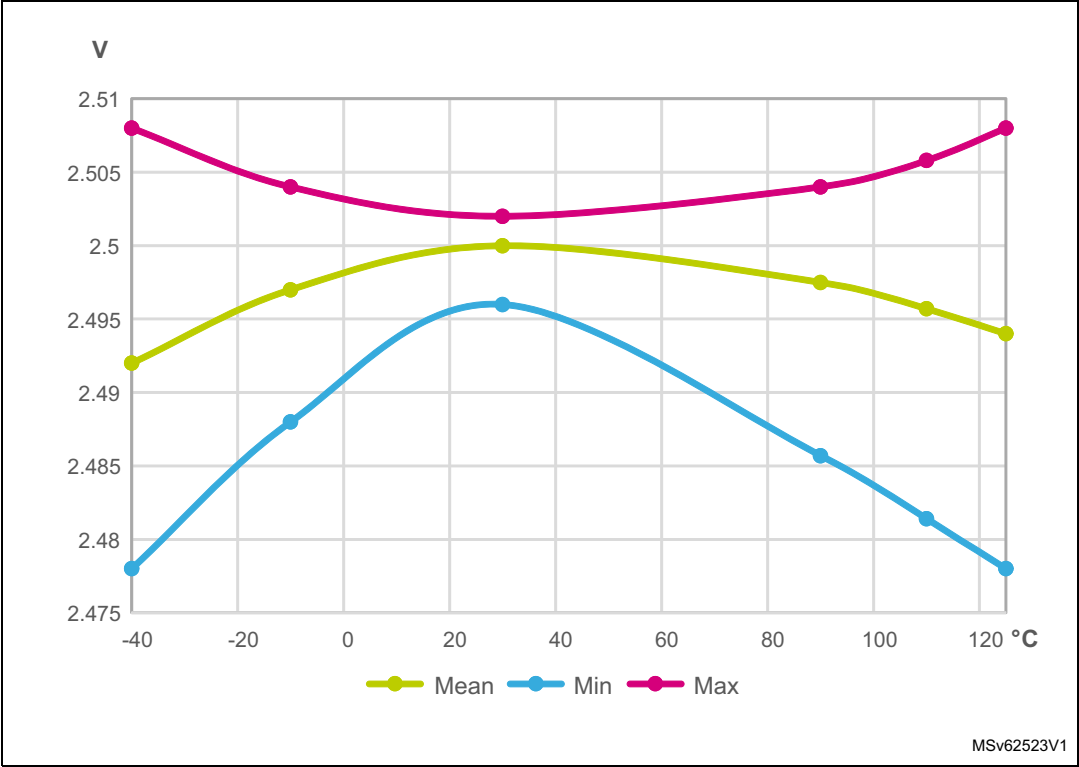
Figure 32. V_{\text{REFOUT}} TEMP in case VRS = 01
