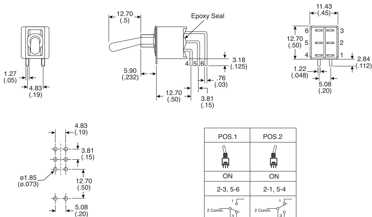
P.C. Mounting
