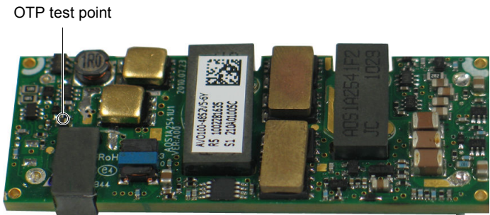
Figure 10 OTP test point
