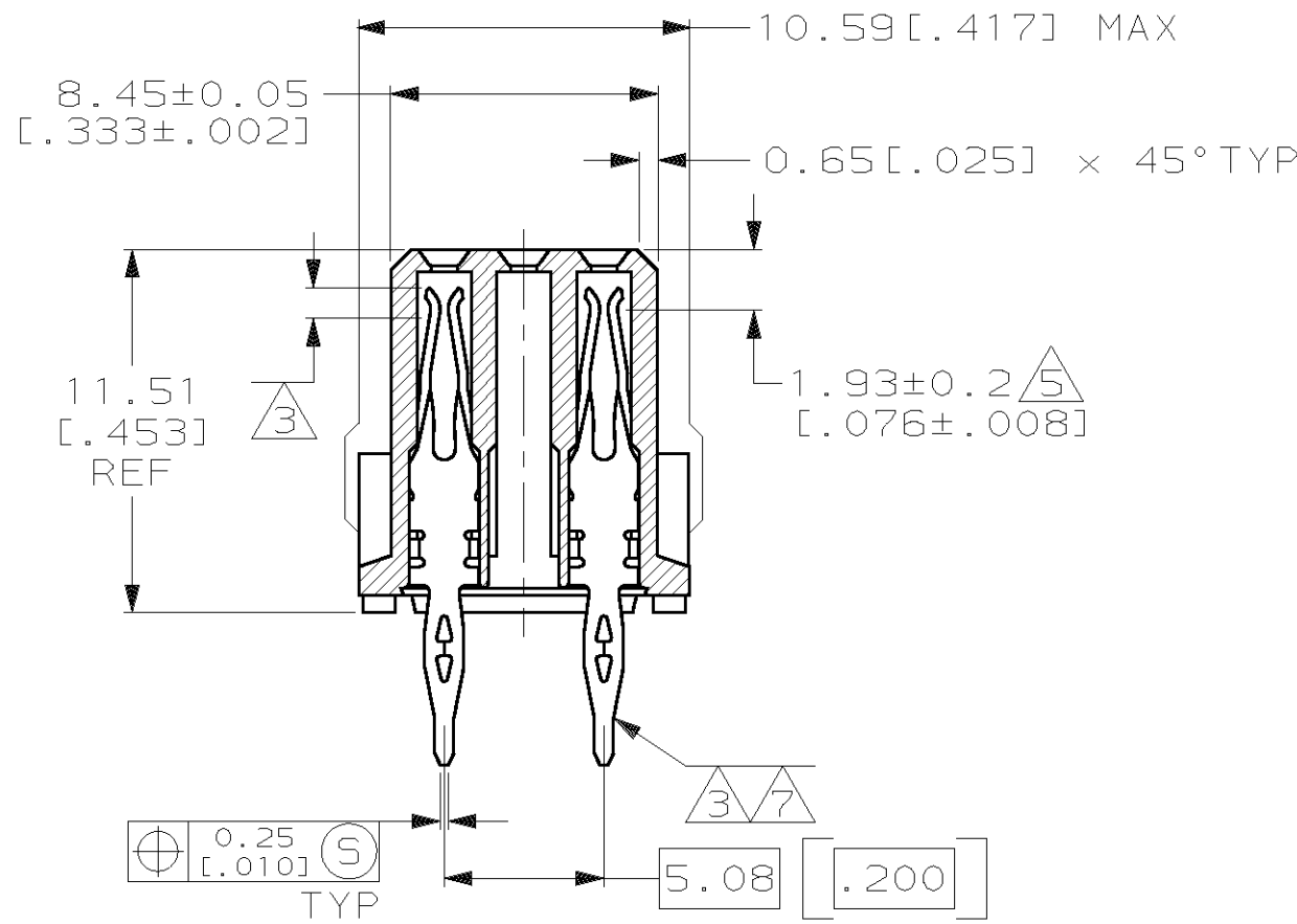
SECTION X-X
