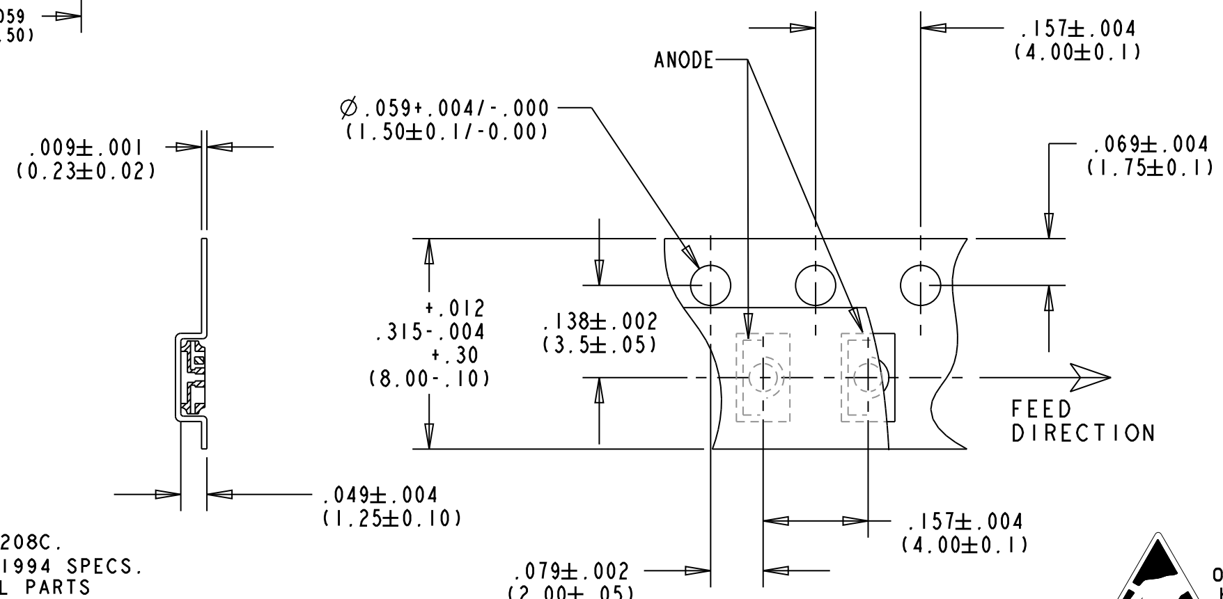
TAPING SPECIFICATION NO SCALE
