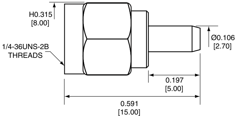
SIDE VIEW
