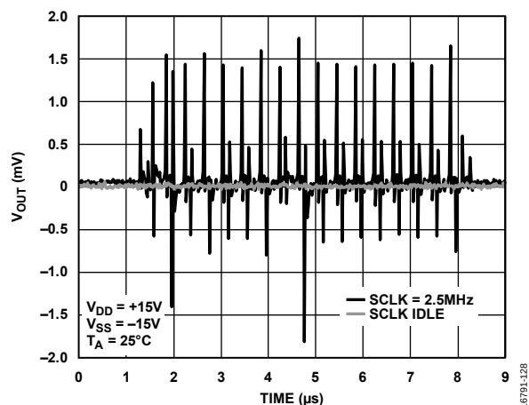
Figure 28. Digital Feedthrough
