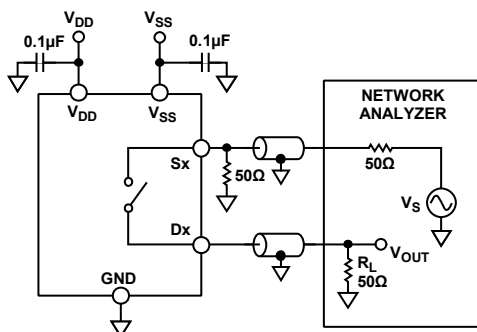
Figure 34. Off Isolation
