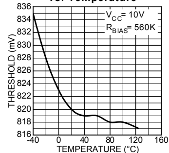
ISNS Current Limit Threshold vs. Temperature
