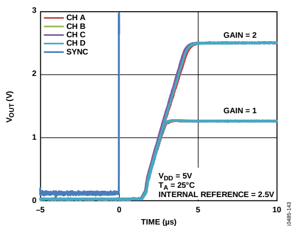
Figure 39. Exiting Power-Down to Midscale
