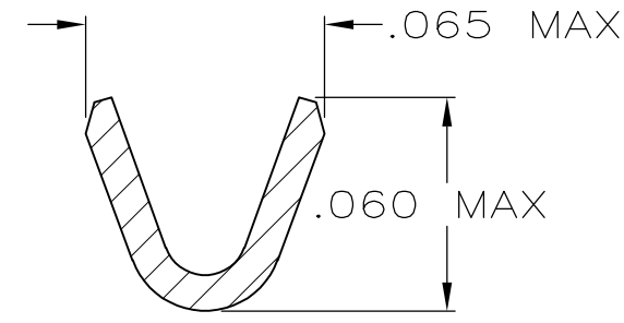
SECTION C-C SCALE 20:1
