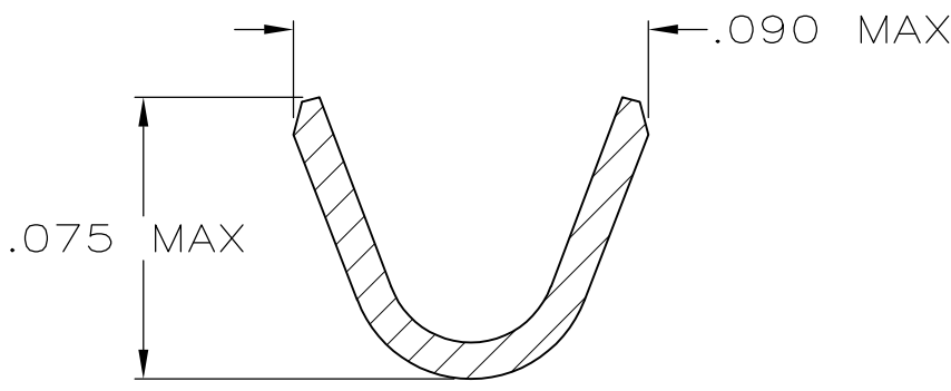
SECTION B-B SCALE 20:1
