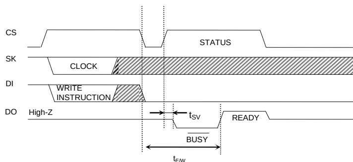
Figure 48. READY/ \overline{\text{BUSY}} STATUS Output Timing Chart
