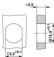
Housing cutout for M16 fastening thread, mounting panel with feed-through hole
