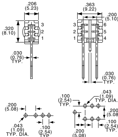
TT11DGVRA3T Vertical Actuation
