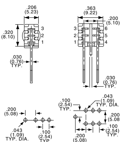
TT21NGVRA1 Vertical Actuation
