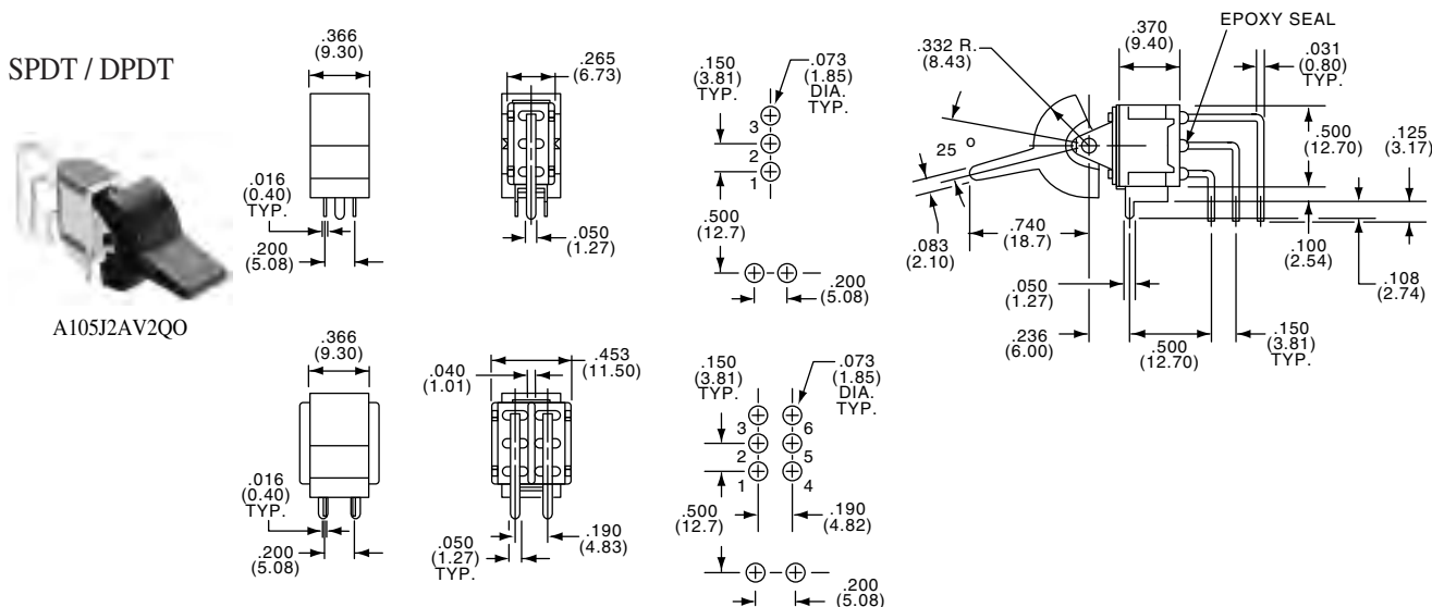
Standard Paddle Color - (Black)
