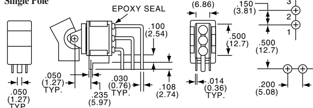
Vertical Right Angle Single Pole
