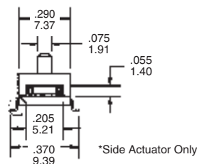
Upright, Surface Mount "L" Type, Extended Actuator
