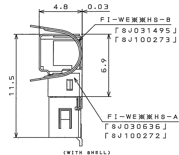
COUNTERPART CONNECTOR (SCALE 4:1)
