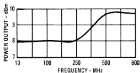
Power Output*
