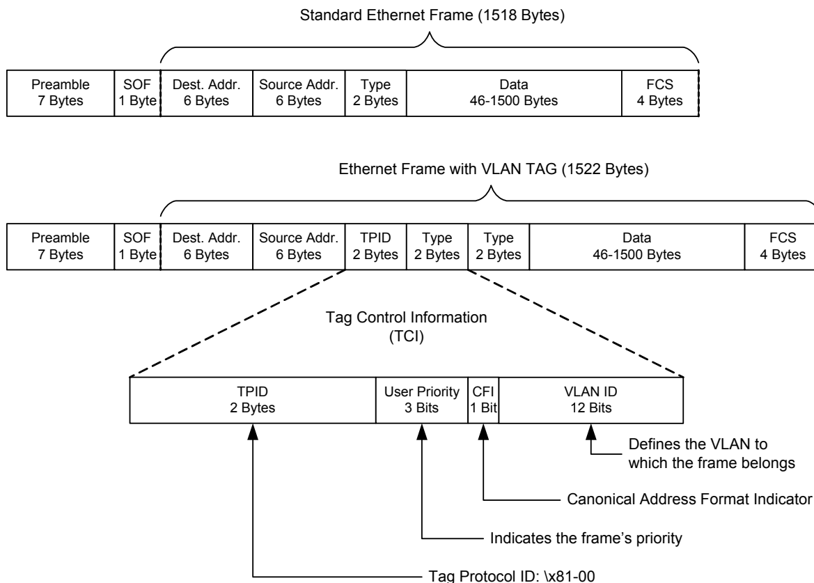
Figure 9.1 VLAN Frame
