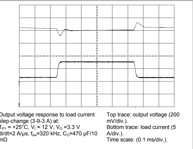
Output Load Transient Response, Default PID/NLR
