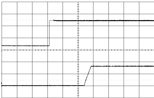
Start-up enabled by connecting V_I at: T_{P1} = +25^{\circ}\text{C} , V_I = 12\text{ V} , V_O = 3.3\text{ V} C_O = 470\text{ }\mu\text{F}/10\text{ m}\Omega , I_O = 12\text{ A} Top trace: Input voltage (5 V/div.). Bottom trace: Output voltage (2 V/div.). Time scale: (20 ms/div.).
