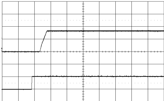
Start-up enabled by connecting V_I at: T_{P1} = +25^{\circ}\text{C} , V_I = 12\text{ V} , V_O = 3.3\text{ V} C_O = 470\text{ }\mu\text{F}/10\text{ m}\Omega , I_O = 12\text{ A} Top trace: output voltage (2 V/div.). Bottom trace: CTRL signal (2 V/div.). Time scale: (20 ms/div.).
