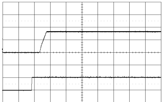
Start-up by enabling CTRL signal at: T_{P1} = +25^{\circ}\text{C} , V_I = 12\text{ V} , V_O = 3.3\text{ V} C_O = 470\text{ }\mu\text{F}/10\text{ m}\Omega , I_O = 12\text{ A} Top trace: output voltage (2 V/div.). Bottom trace: CTRL signal (2 V/div.). Time scale: (20 ms/div.).
