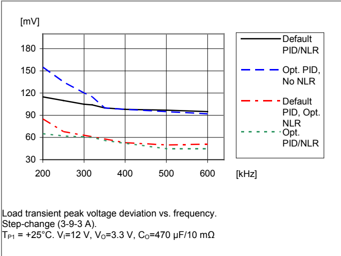
Load transient vs. Switch Frequency
