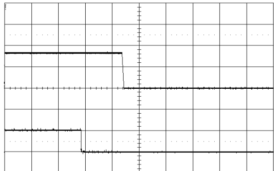
Shut-down enabled by disconnecting V_I at: T_{P1} = +25^{\circ}\text{C} , V_I = 12\text{ V} , V_O = 3.3\text{ V} C_O = 470\text{ }\mu\text{F}/10\text{ m}\Omega , I_O = 12\text{ A} Top trace: output voltage (2 V/div.). Bottom trace: CTRL signal (2 V/div.). Time scale: (2 ms/div.).
