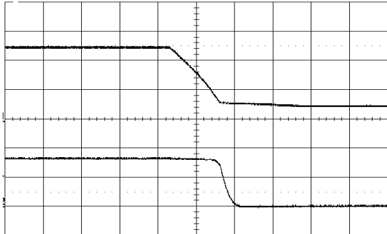
Shut-down enabled by disconnecting V_I at: T_{P1} = +25^{\circ}\text{C} , V_I = 12\text{ V} , V_O = 3.3\text{ V} C_O = 470\text{ }\mu\text{F}/10\text{ m}\Omega , I_O = 12\text{ A} Top trace: Input voltage (5 V/div.). Bottom trace: Output voltage (2 V/div.). Time scale: (2 ms/div.).
