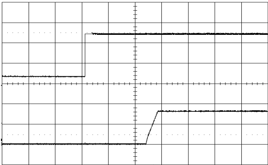
Start-up enabled by connecting V_I at: T_{P1} = +25^{\circ}\text{C} , V_I = 12\text{ V} , V_O = 3.3\text{ V} C_O = 470\text{ }\mu\text{F}/10\text{ m}\Omega , I_O = 12\text{ A} Top trace: Input voltage (5 V/div.). Bottom trace: Output voltage (2 V/div.). Time scale: (20 ms/div.).
