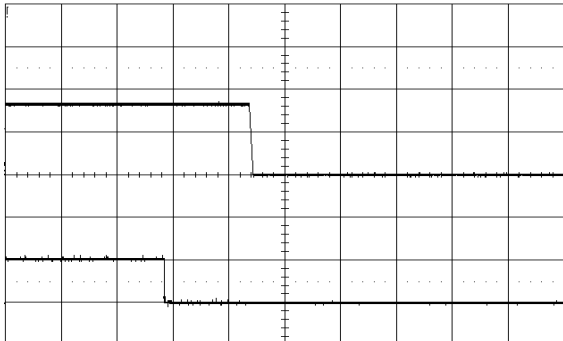
Shut-down enabled by disconnecting V_I at: T_{P1} = +25^{\circ}\text{C} , V_I = 12\text{ V} , V_O = 3.3\text{ V} C_O = 470\text{ }\mu\text{F}/10\text{ m}\Omega , I_O = 12\text{ A} Top trace: output voltage (2 V/div.). Bottom trace: CTRL signal (2 V/div.). Time scale: (2 ms/div.).
