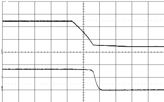
Shut-down enabled by disconnecting V_I at: T_{P1} = +25^{\circ}\text{C} , V_I = 12\text{ V} , V_O = 3.3\text{ V} C_O = 470\text{ }\mu\text{F}/10\text{ m}\Omega , I_O = 12\text{ A} Top trace: Input voltage (5 V/div.). Bottom trace: Output voltage (2 V/div.). Time scale: (2 ms/div.).
