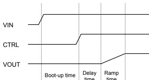
Illustration of Power Up Procedure.
