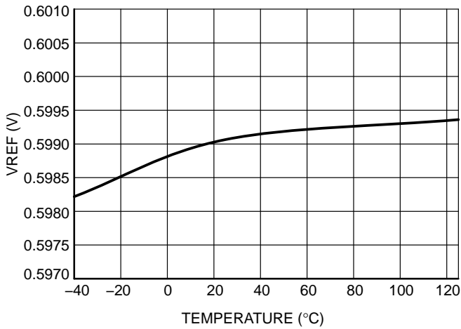
Figure 10. V_{\text{REF}} vs T at V_{\text{HVBIAS}} = 48\text{ V}
