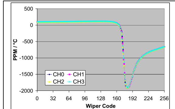
FIGURE 2-19: 5\text{ k}\Omega – R_{WB} PPM/ ^\circ\text{C} vs. Wiper Setting. ( R_{BW(\text{code}=n, 125^\circ\text{C})} - R_{BW(\text{code}=n, -40^\circ\text{C})} / R_{BW(\text{code}=256, 25^\circ\text{C})} / 165^\circ\text{C} * 1,000,000 ) ( V_{DD} = 3.0\text{V} , I_W = 190\text{ }\mu\text{A} ).
