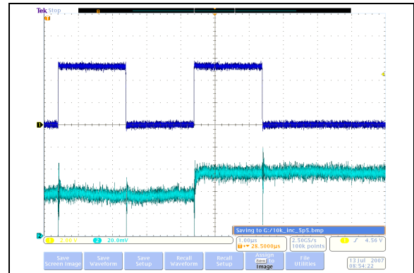
FIGURE 2-44: 10 kΩ – Low-Voltage Increment Wiper Settling Time ( V_{DD} = 5.5\text{V} ) (1 μs/Div).
