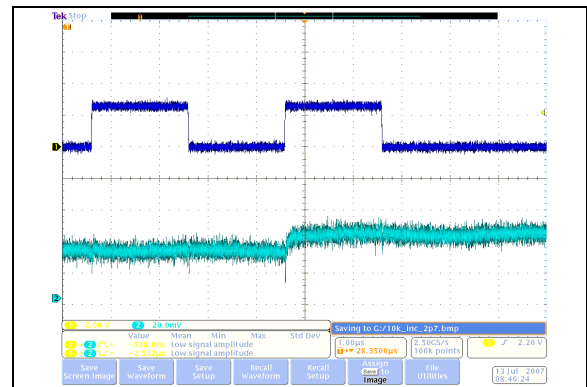
FIGURE 2-45: 10 kΩ – Low-Voltage Increment Wiper Settling Time ( V_{DD} = 2.7\text{V} ) (1 μs/Div).
