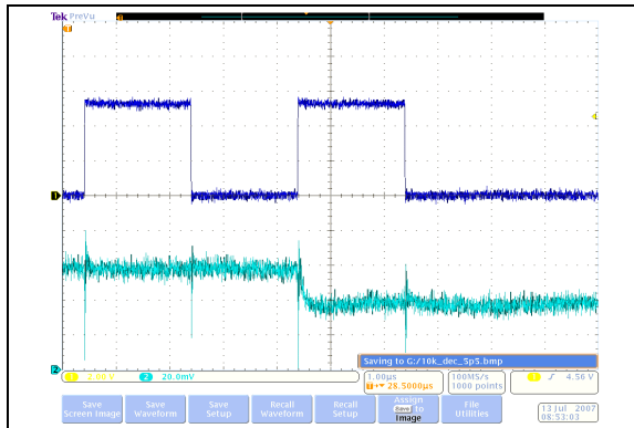
FIGURE 2-42: 10 kΩ – Low-Voltage Decrement Wiper Settling Time ( V_{DD} = 5.5\text{V} ) (1 μs/Div).
