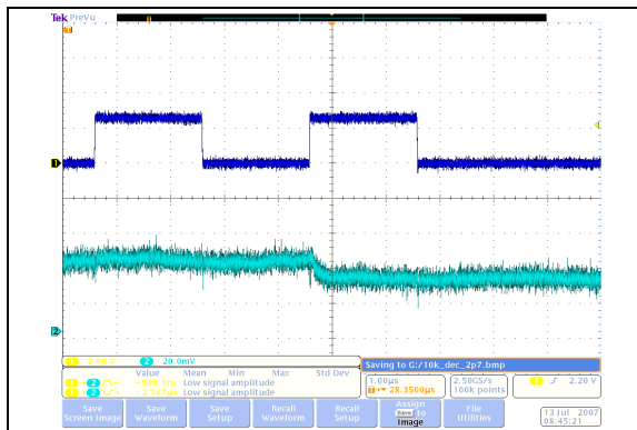
FIGURE 2-43: 10 kΩ – Low-Voltage Decrement Wiper Settling Time ( V_{DD} = 2.7\text{V} ) (1 μs/Div).
