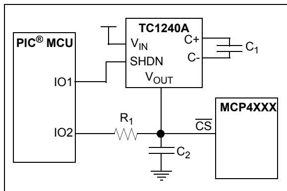
FIGURE 8-3: Using the TC1240A to Generate the V_{IHH} Voltage.
