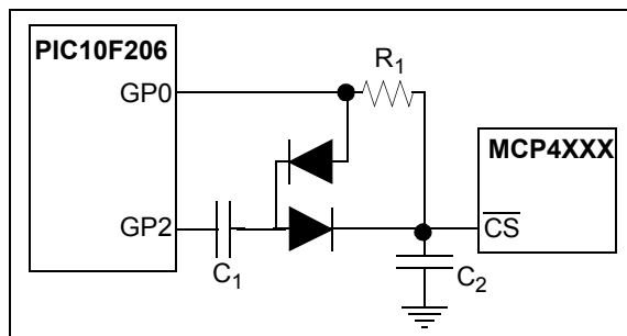
FIGURE 8-4: MCP4XXX Nonvolatile Digital Potentiometer Evaluation Board (MCP402XEV) implementation to generate the V_{IHH} voltage.
